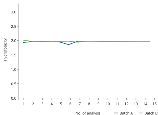
Hydrofobicity test
